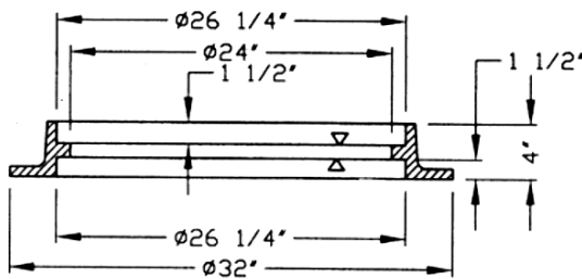
FRAME SECTION - XX
