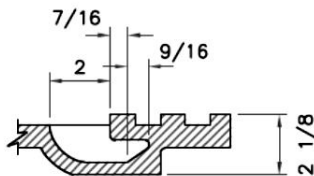
SECTION THROUGH PICK HOLE
