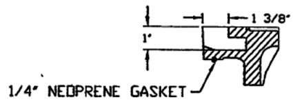
PICK HOLE DETAIL
