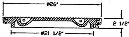
COVER SECTION
