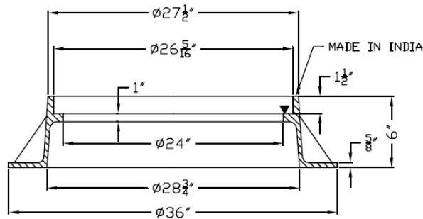
Frame Section View
