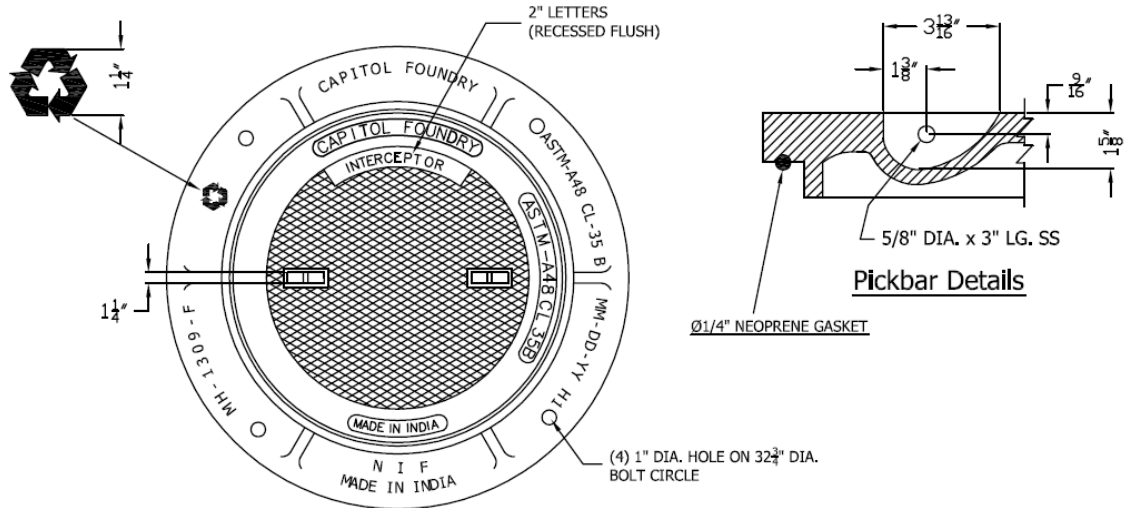
Top view (Assembly)
