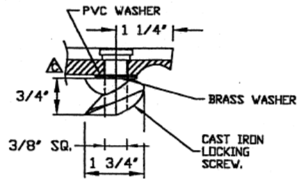
LOCK DETAIL
