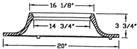
SECTION-XX
