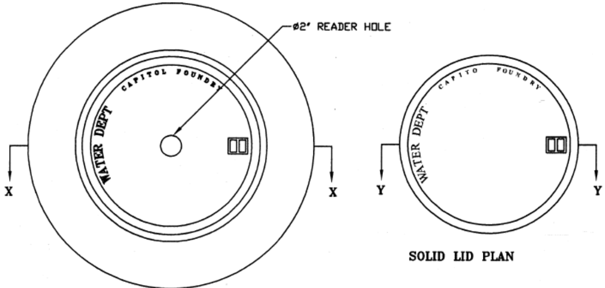
PLAN(WITH HOLE LID)
