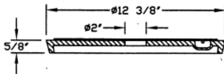
HOLE LID SECTION-XX
