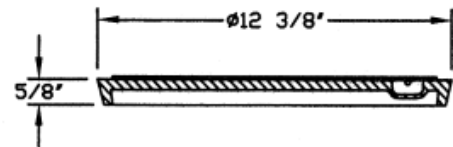
SECTION-YY
