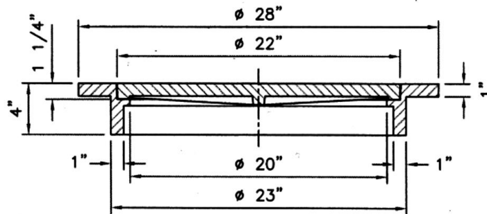
SECTION XX.
