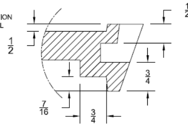
SECTION A-A DETAIL
